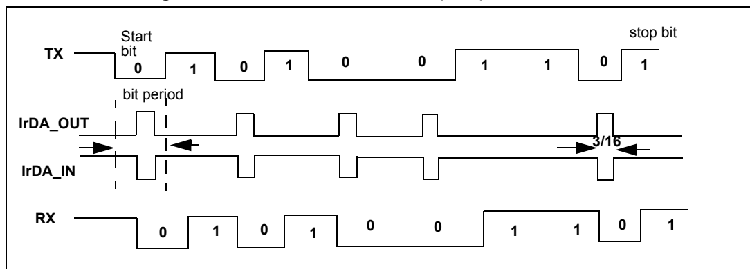
Figure 314. IrDA data modulation (3/16) -Normal mode
