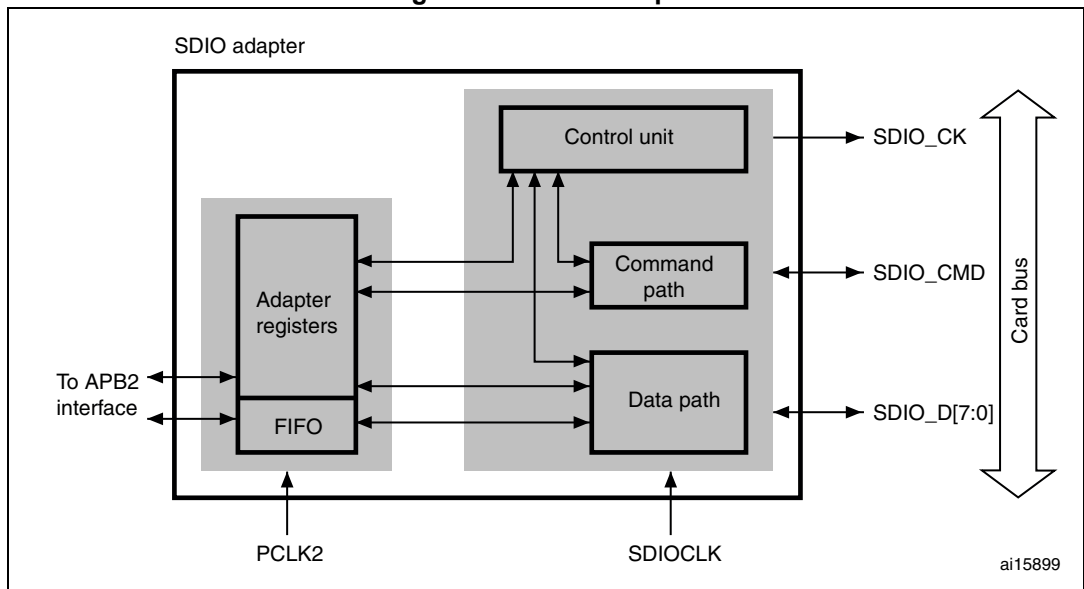
Figure 327. SDIO adapter
