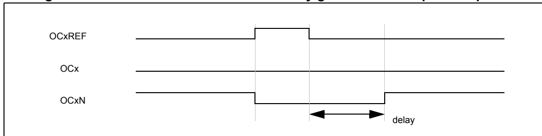
Figure 122. Dead-time waveforms with delay greater than the positive pulse.
