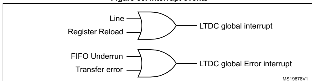
Figure 85. Interrupt events
