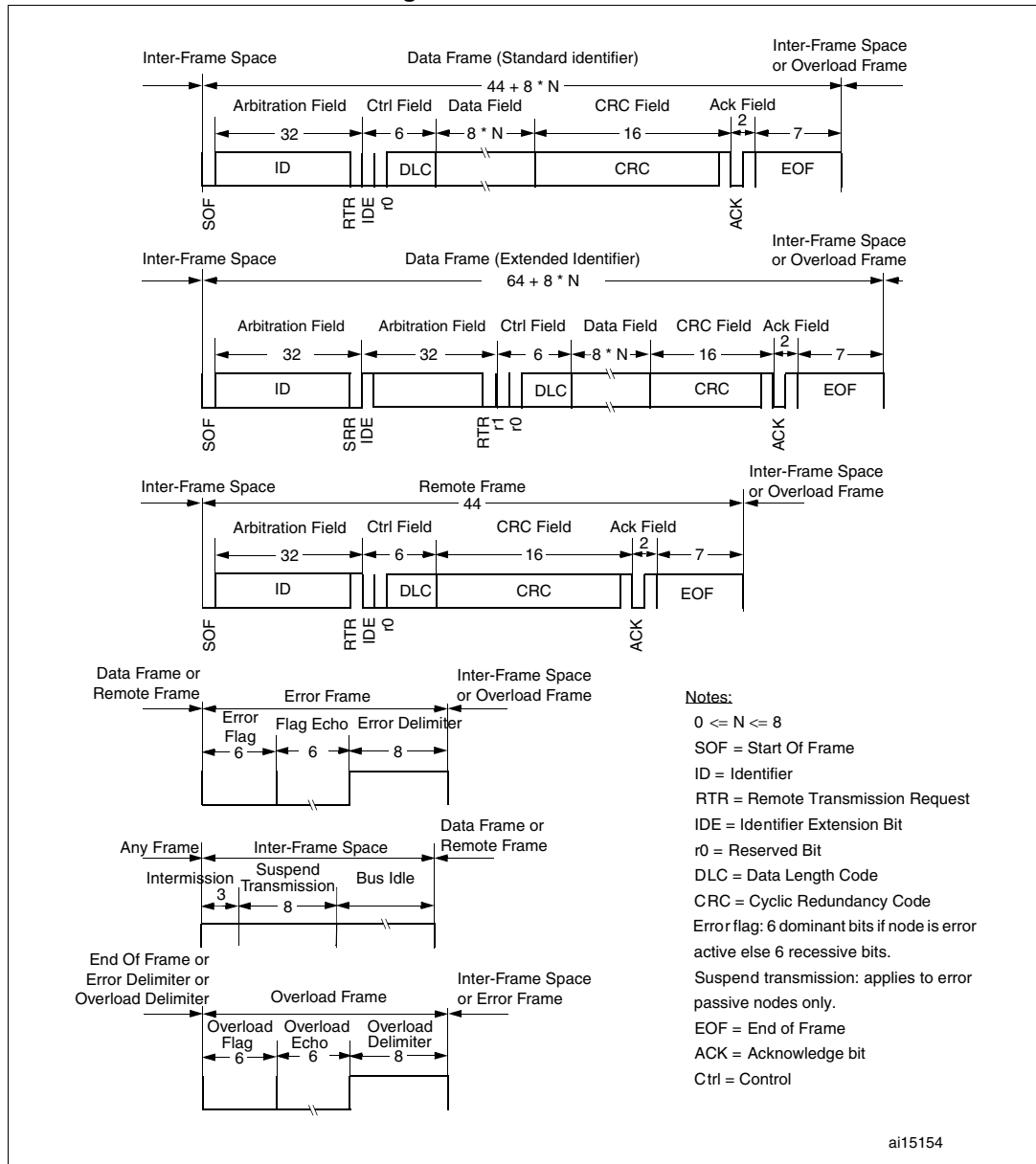
Figure 347. CAN frames
