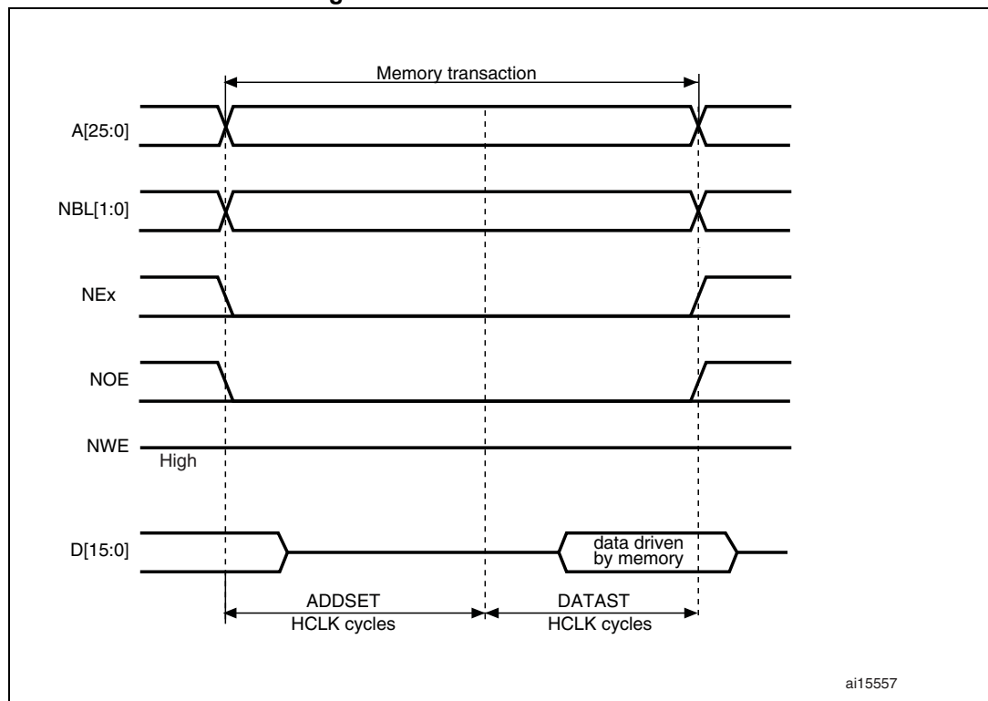
Figure 434. Mode1 read accesses
