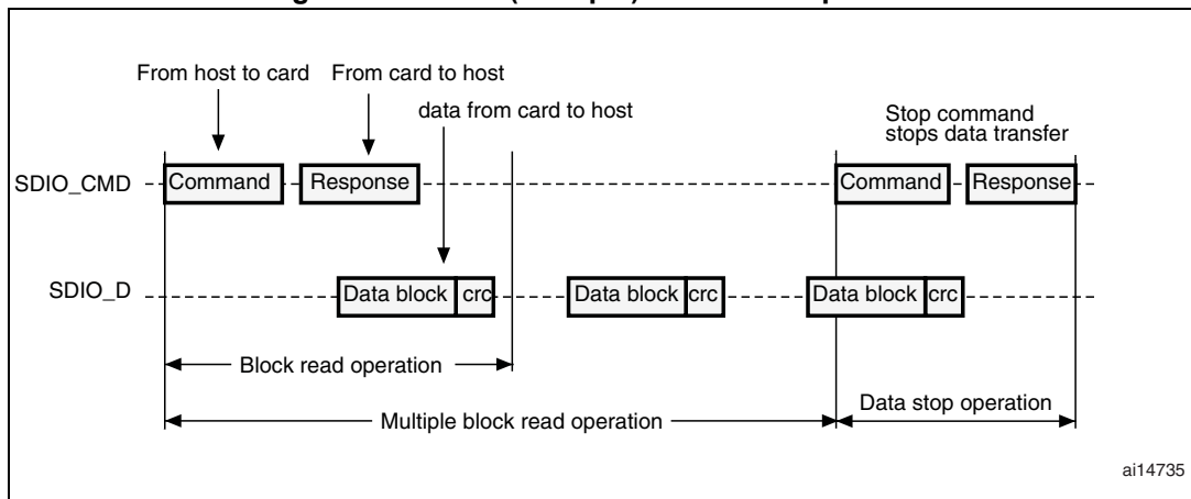
Figure 322. SDIO (multiple) block read operation
