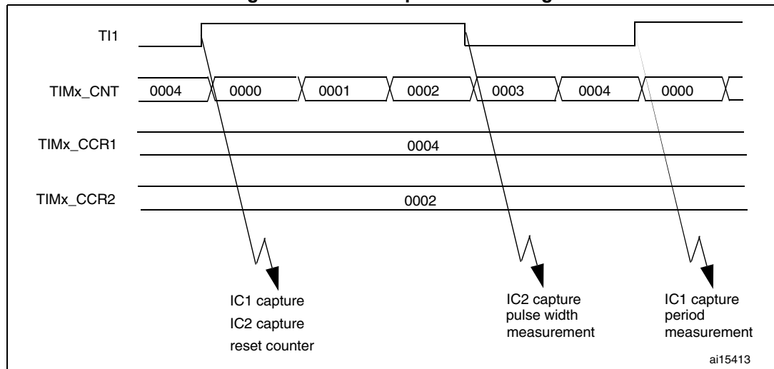
Figure 196. PWM input mode timing
