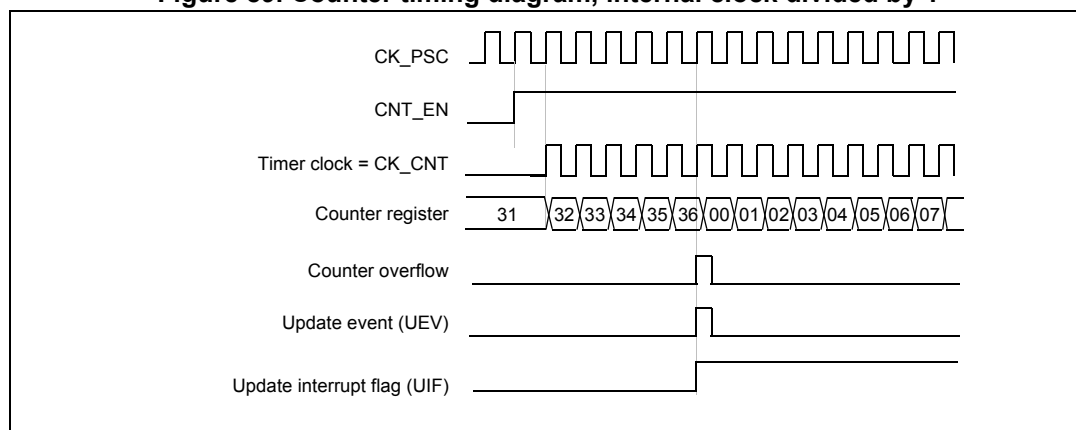
Figure 89. Counter timing diagram, internal clock divided by 1
