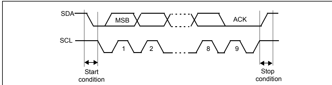
Figure 238. I 2 C bus protocol
