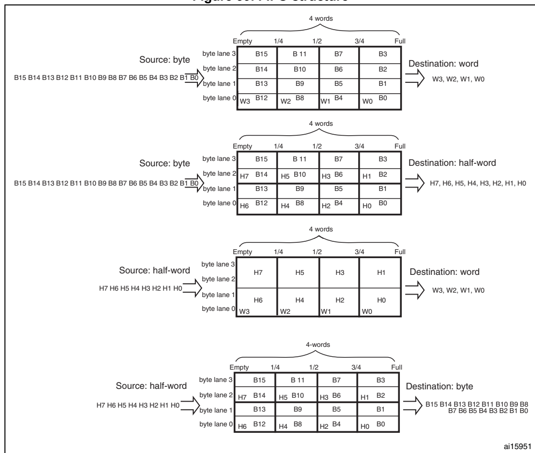
Figure 39. FIFO structure
