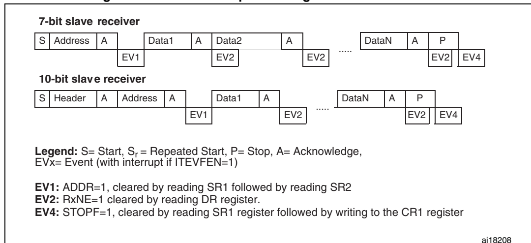
Figure 242. Transfer sequence diagram for slave receiver
