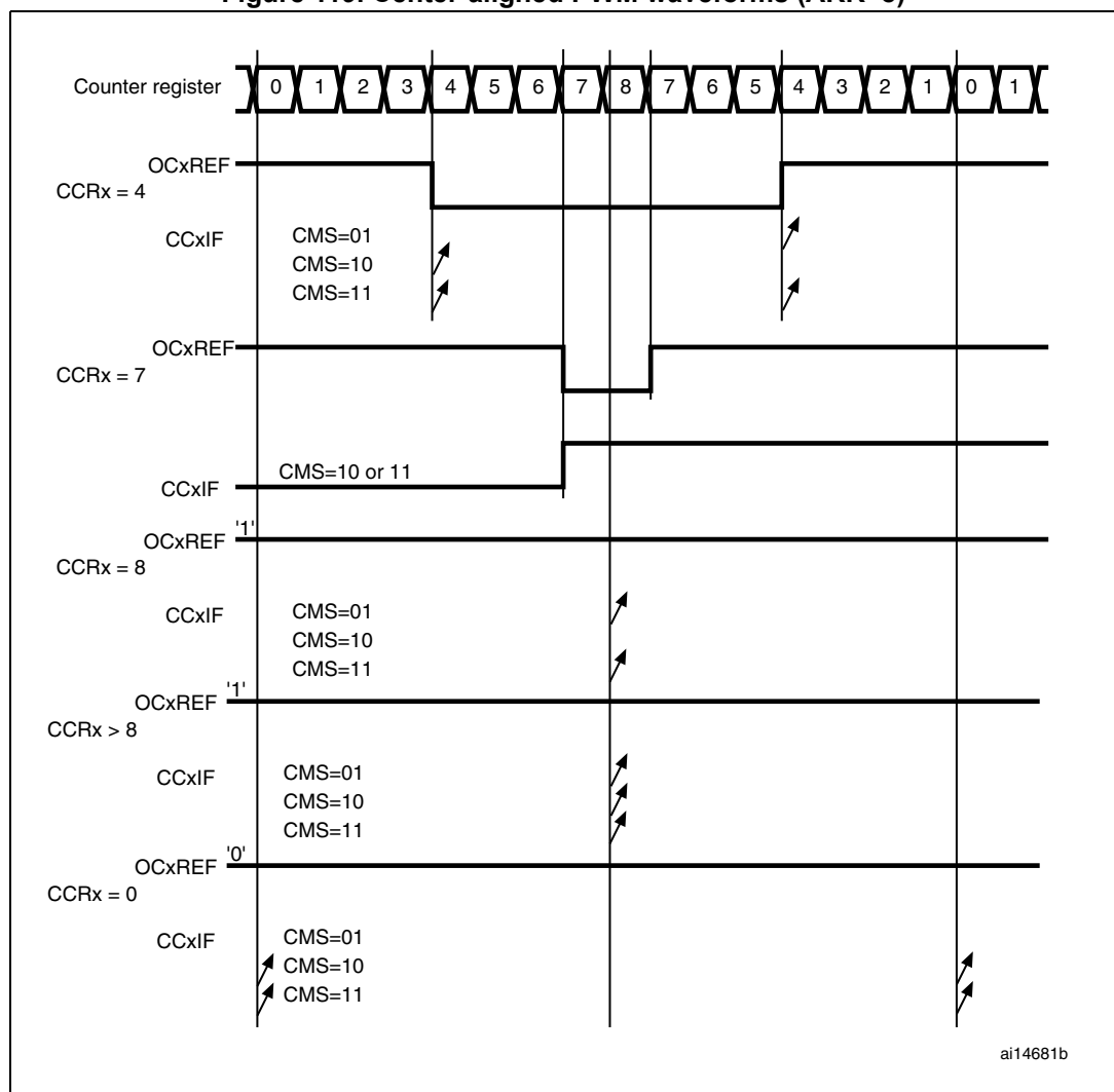
Figure 119. Center-aligned PWM waveforms (ARR=8)
