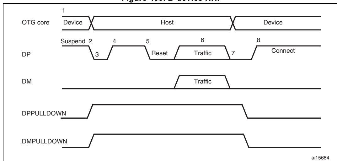
Figure 409. B-device HNP
