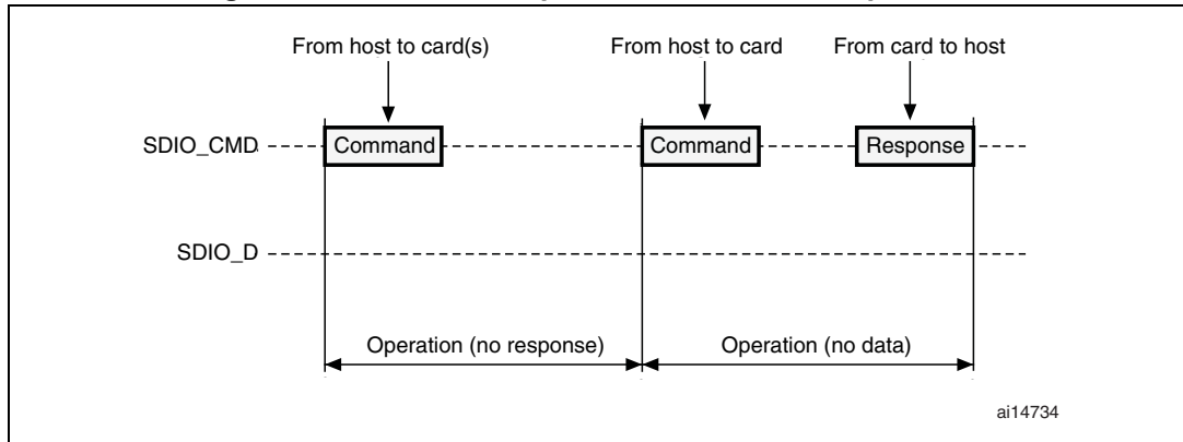
Figure 321. SDIO “no response” and “no data” operations
