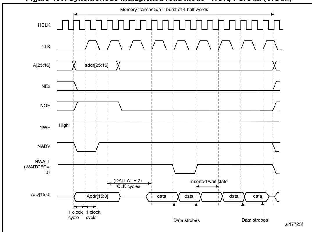
Figure 450. Synchronous multiplexed read mode - NOR, PSRAM (CRAM)
