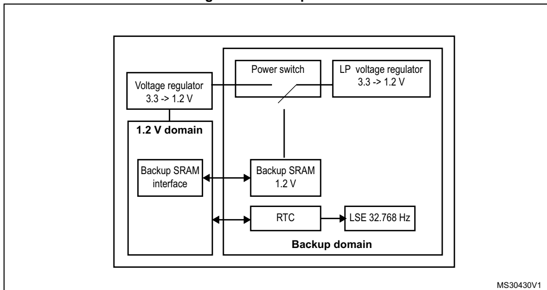
Figure 11. Backup domain
