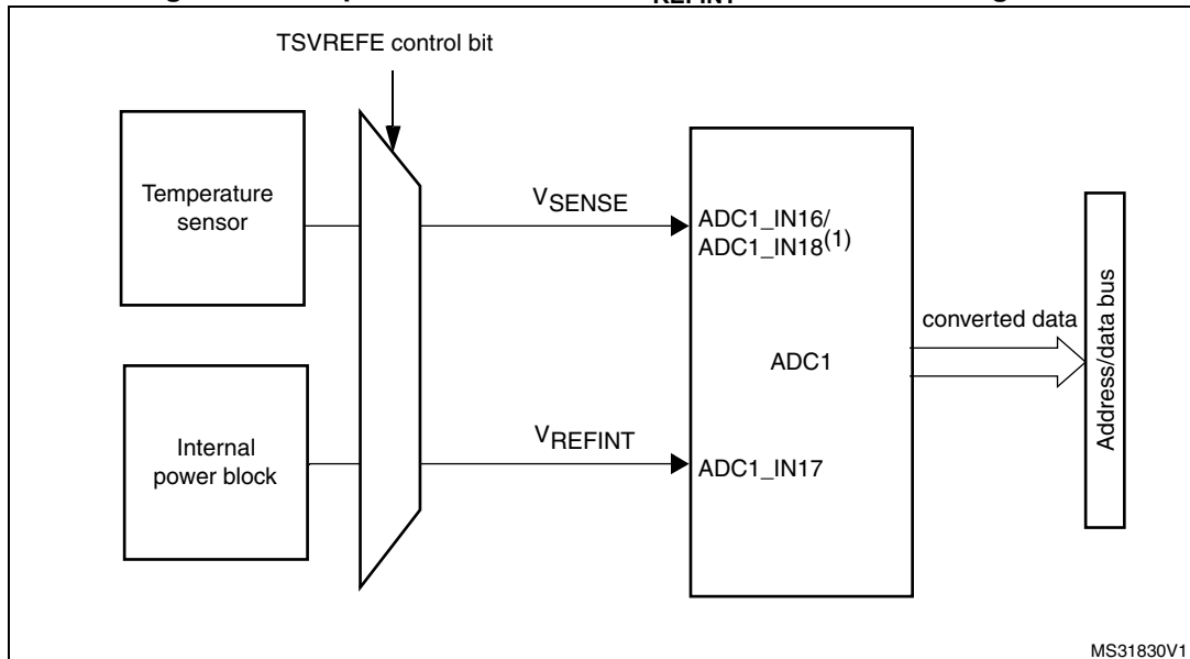
Figure 63. Temperature sensor and V_{REFINT} channel block diagram
